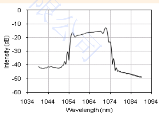
Optical Spectrum Corresponding to a Chirped Pulse Width of 0.2 ps
