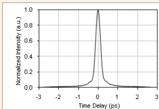
Autocorrelation Trace Corresponding to a Chirped Pulse Width of 0.2 ps
