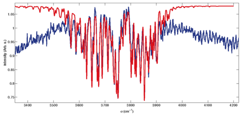
H 2 O absorption lines red: theoretical (Hitran simulation) - blue: experimental
