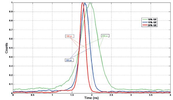
Timing jitter (ps) vs QE (%)
