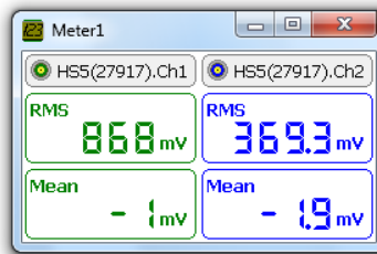
Figure 2.7: Voltmeter.
