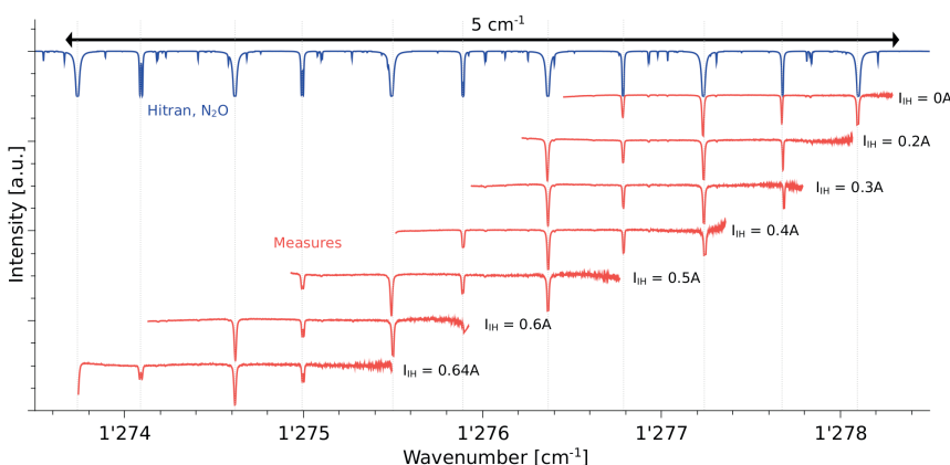
Example of wide scanning of a \text{N}_2\text{O} gas cell, with fast I_L scans and independent I_T values.
