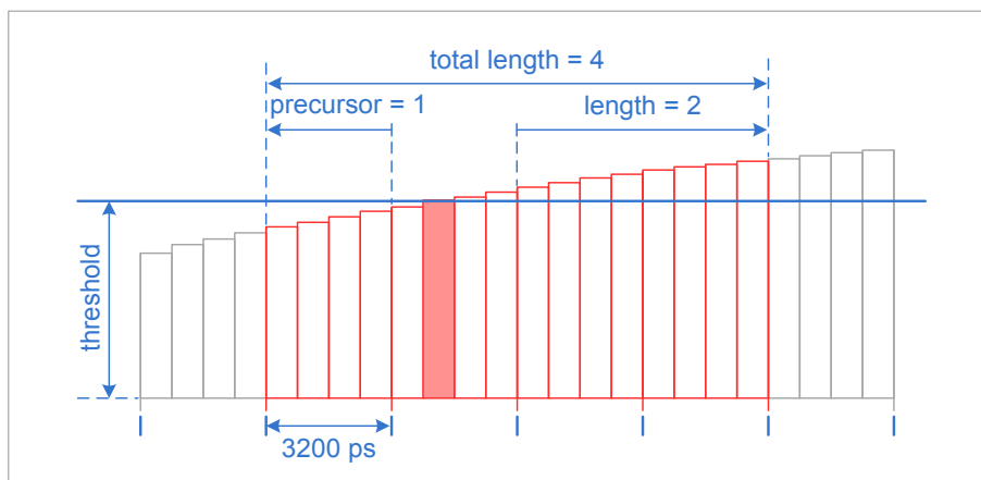
Figure 2.13: Triggering in 4 channel mode at 4 samples per clock cycle.
