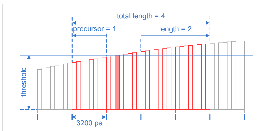
Figure 2.14: Triggering in 2 channel mode at 8 samples per clock cycle.
