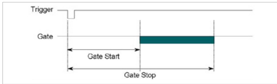
Figure 2.21: Gate and delay functionality: When a trigger occurs, the gate opens after a set period of time ("gate start") and closes when it reaches "gate stop".
