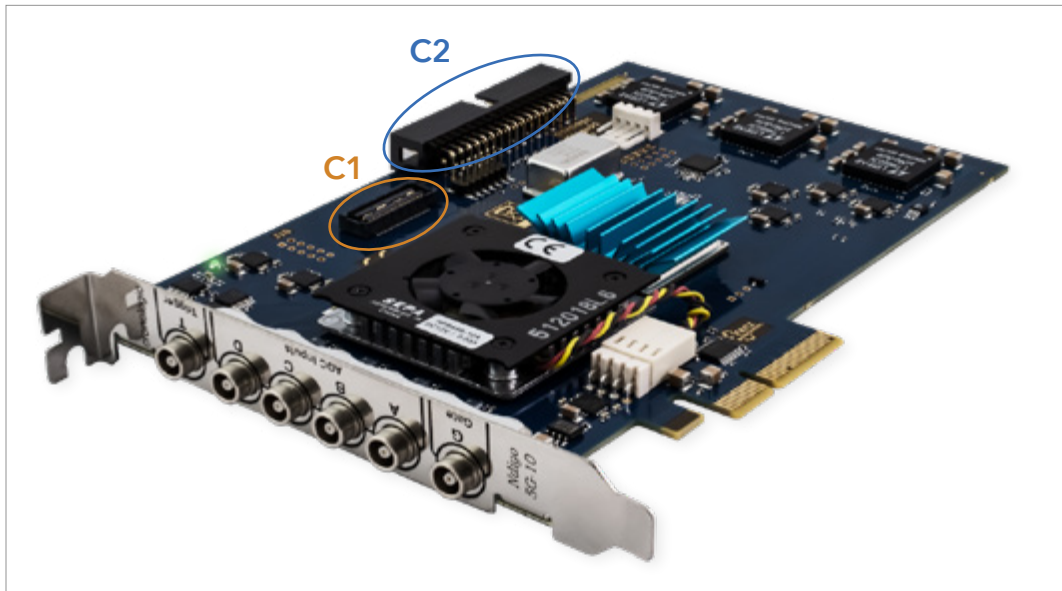
Figure 2.3: Ndigo5G board showing inter-board connectors C1 and C2.
