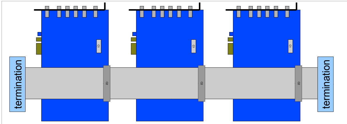
Figure 2.1: If several Ndigo boards are connected to work in sync, the boards must be connected using a ribbon cable as bus for synchronization and trigger signals. Proper termination is required at both ends of the cable.
