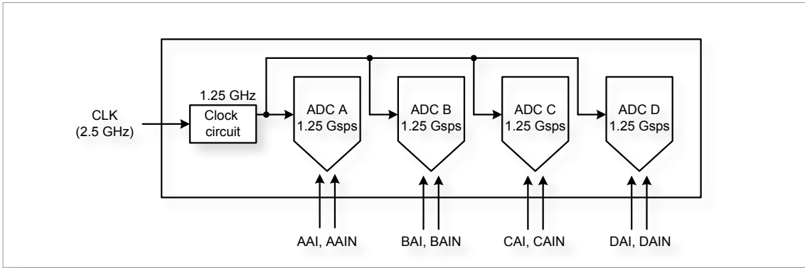
Figure 2.7: ADCs in 4 channel mode ABCD at 1.25Gps.
