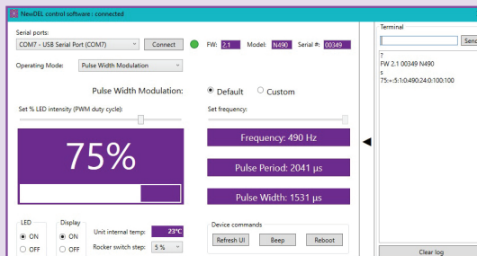
SOFTWARE INTERFACE
