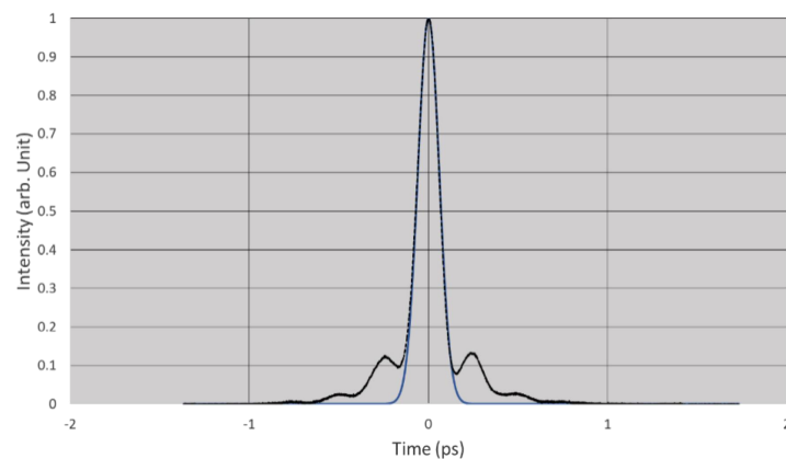
Autocorrelation Trace and Gaussian fit-TFWHM= 99 fs
