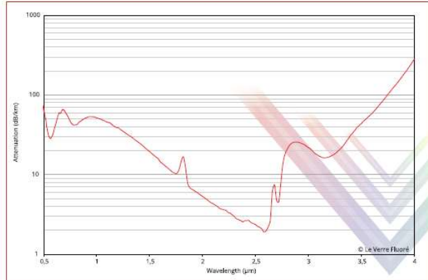
Typical 6,5/125 \mu\text{m} ZFG single mode fiber attenuation
