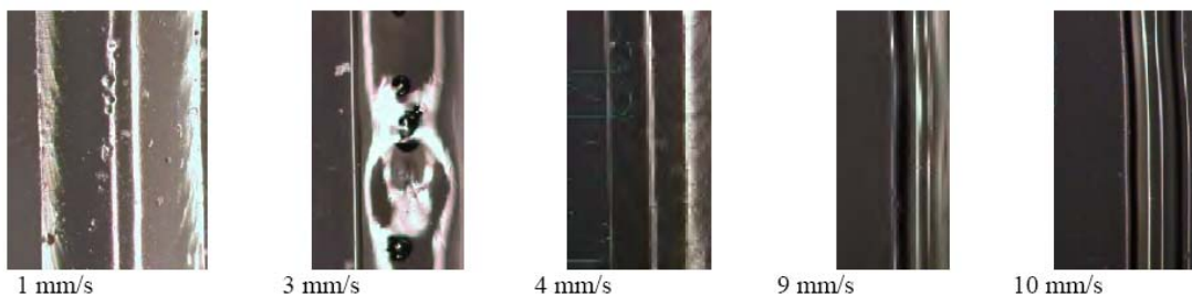
Figure. 6 Optical microscope images of the lines of melted PMMA material made on surface of the sample with different scanning speeds. The laser power – 3.45 W.
