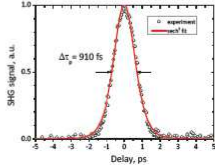
Autocorrelation trace at maximum power
