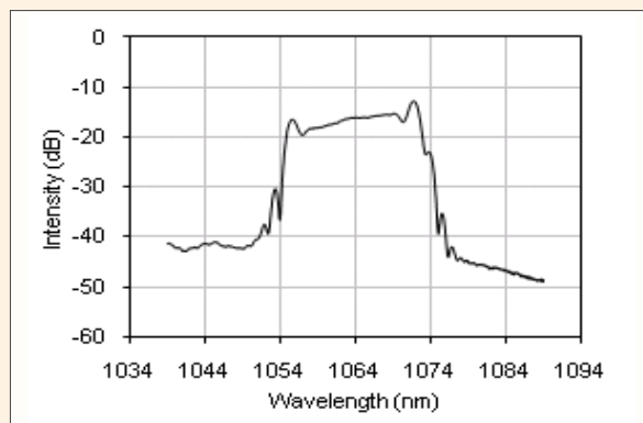
Optical Spectrum Corresponding to a Chirped Pulse Width of 0.2 ps
