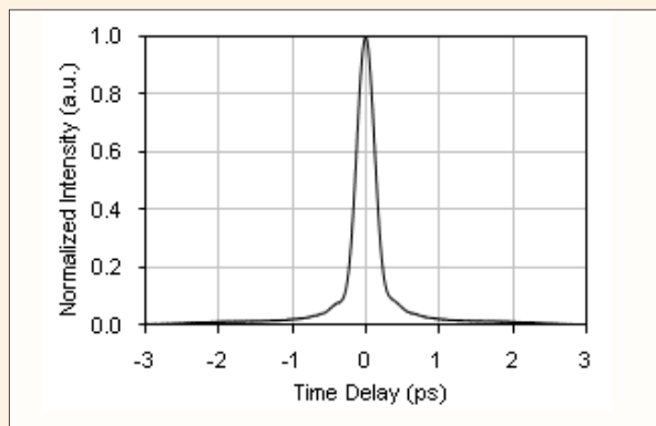
Autocorrelation Trace Corresponding to a Chirped Pulse Width of 0.2 ps
