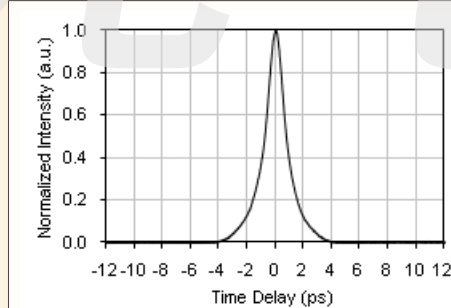
Typical Autocorrelation Trace. Pulse Width = 1 ps
