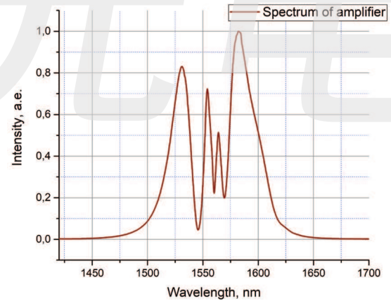
PERL-PM series typical spectrum sample (linear scale)
