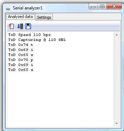
Figure 9.4: Serial analyzer output window
