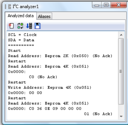
Figure 9.3: I 2 C analyzer output window
