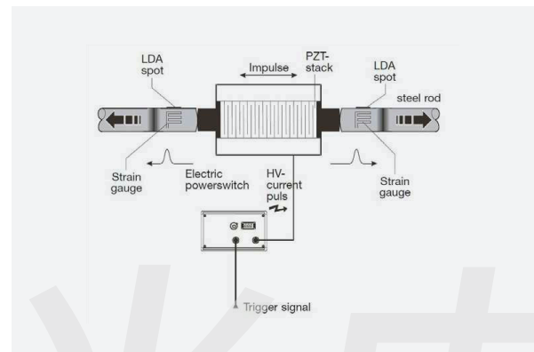
Figure 2: Symmetrical piezo-shock-generator with two-side shock propagation. The shock parameters are detected by strain gauges & LDAs.
