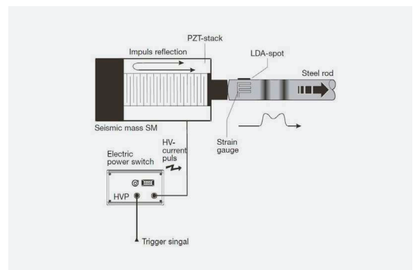
Figure 7: Schematic of a single end piezo-shock-generated system by application of a seismic mass. The interaction of travelling pulses results in an elongated double pulse output.
