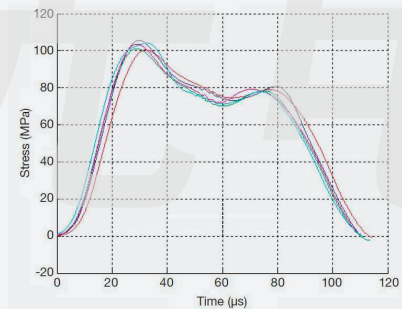
Figure 11: Mechanical stress/time profile time for a burst of shocks. Active stack length: 120 mm. Shockwave energy: 3.25J.
