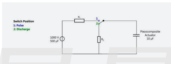
Figure 12: Schematic of piezo-actuator by a HighVoltagePulser (HVP).
