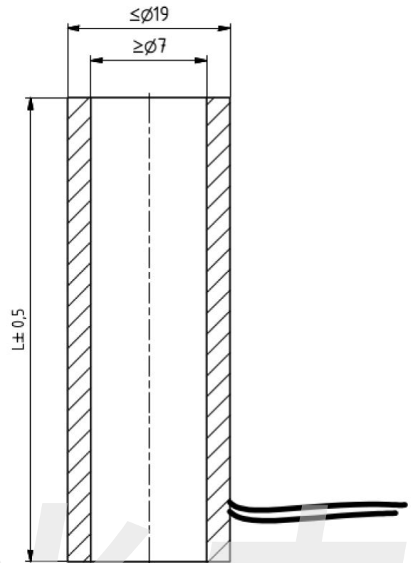
Technical drawing of HPSt 15-8 series
