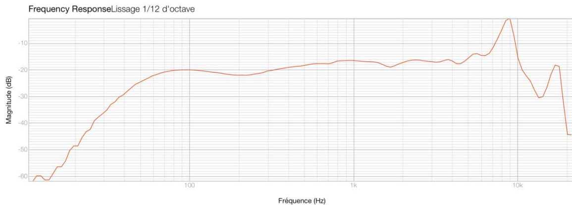
Frequency response measured thanks to B&K type 4232 anechoic test box
