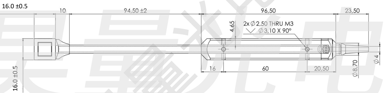
Figure 16: Probe – dimensions (all dimensions are in mm).
