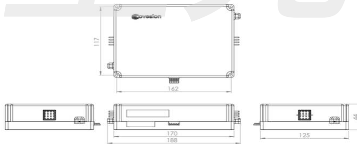
Engineering drawing (mm)
