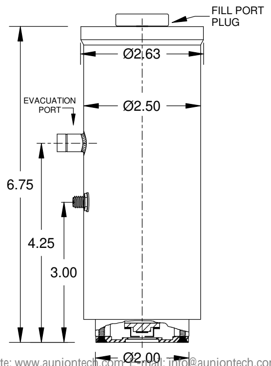
SIDE VIEW MDL-12
