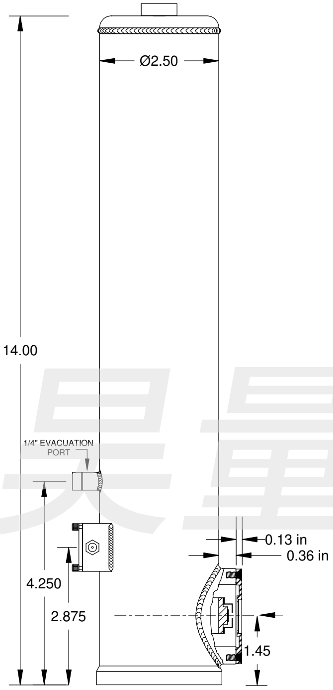
SIDE VIEW MSL-24
