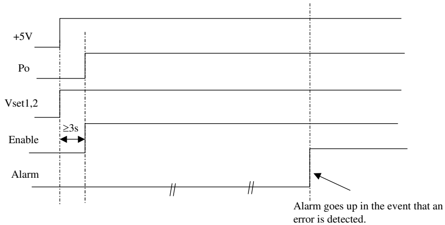
Figure 3 Startup and operational timing of IPSDW0825 module
