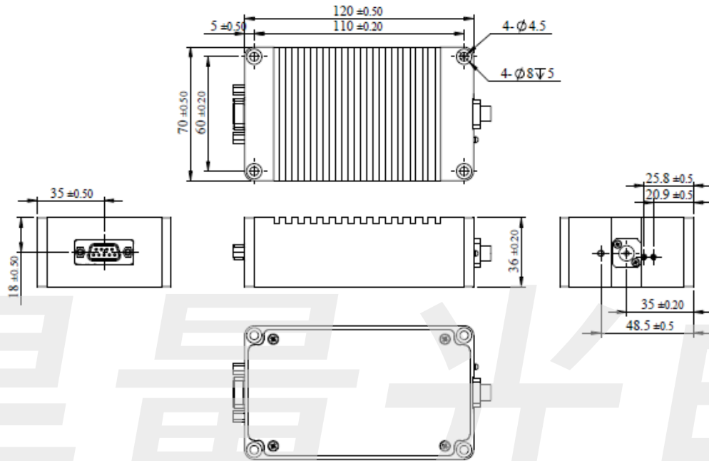
Figure 2 Mechanical drawing of IPSDW0825-0314 module
