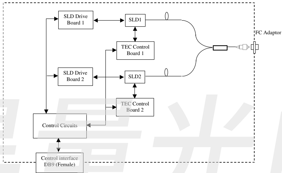
Figure 1 Configuration of IPSDW0825-xxxxx SLD light source module
