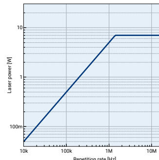
Laser power vs. repetition rate
